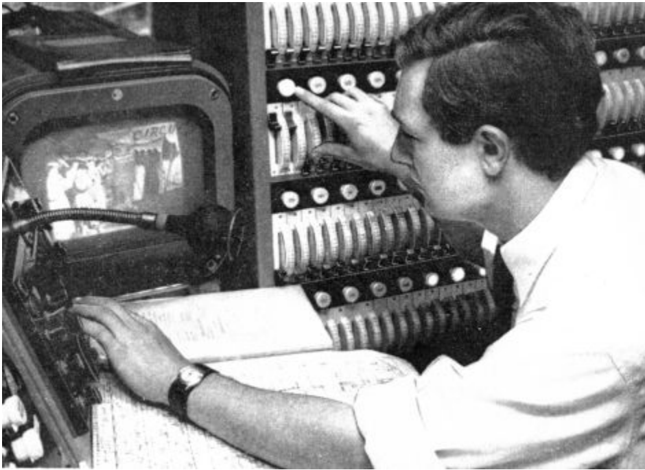
Lighting supervisor using Strand System C Control at the BBC Riverside Studios. From TABS, March 1969.
